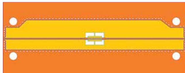
▲ Fig. 4 Prototype microstrip transmission line with an optimized DGS bandstop feature to provide good passband return loss and high rejection at 8.4 GHz.
