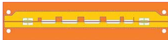
▲ Fig. 5 Final microstrip DGS LPF circuit design, including the transmission line structure for enhanced rejection at 8.4 GHz.
