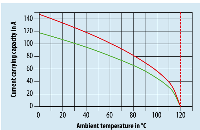
Insert 656.163.706.152.005 with 656.163.806.152.005 equipped with contact diameter 6.0 mm (cable cross-section 16 \text{ mm}^2 ).
