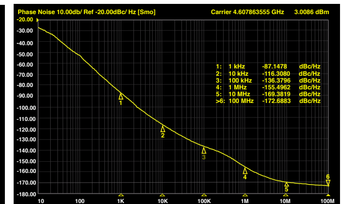
ROS-4608C-X+ Typical Phase Noise
